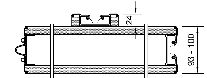
3. JUNCTION PANEL (EE)
